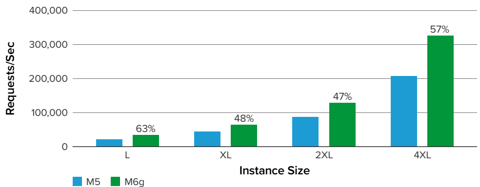
Performance Gain for M6g Versus M5 AMIs for Reverse Proxying with HS256 JWT-Based Authentication
